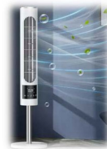
Negative ions
